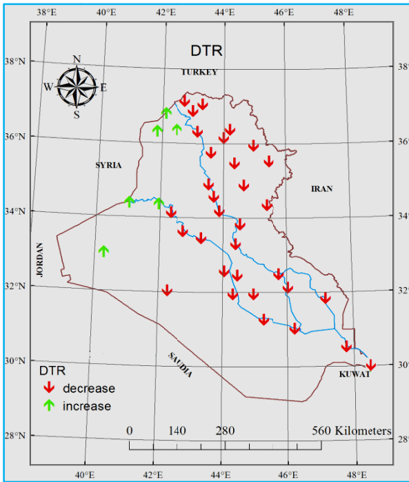
Fig. 5. Extreme temperature index DTR in Iraq during the period 1981-2017
