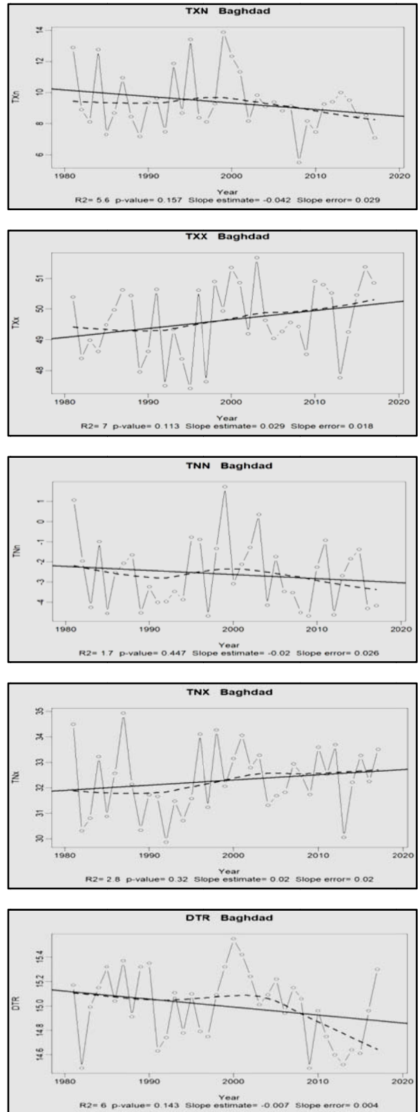
Fig. 2. Five indices of extreme temperature for Baghdad station
