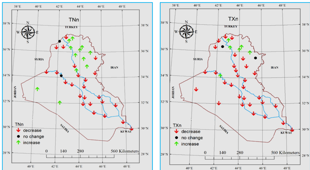
Fig. 4. Annual extreme temperature indices TXn and TNn trends of in Iraq during the period 1981-2017
