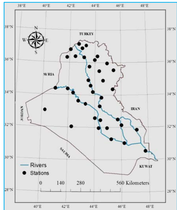
Fig. 1. Map of Iraq with the geographical locations of the stations
