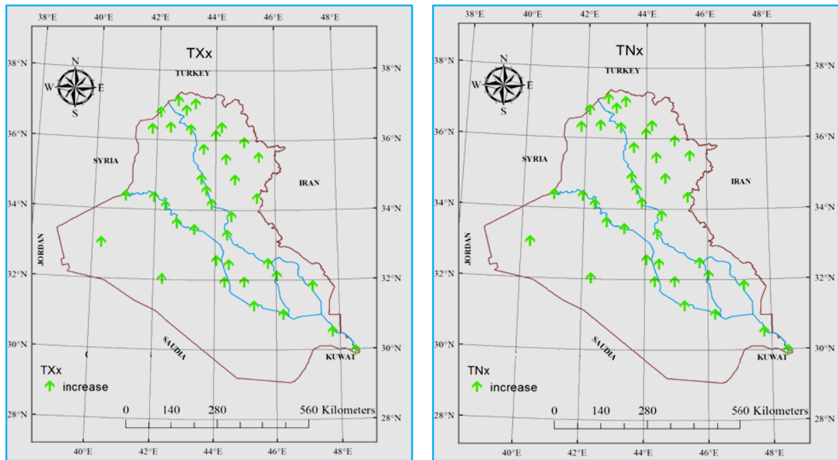
Fig. 3. Monthly extreme temperature indices TXx and TNx trends of in Iraq during the period 1981-2017
