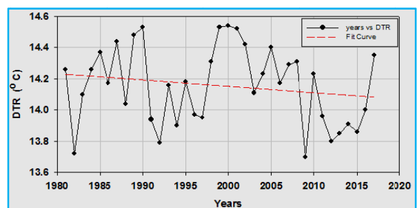
Fig. 6. Time series curves of annual indices over Iraq during 1981-2017
