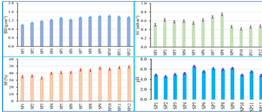
Fig. 3. Distribution of bulk density (BD), soil electrical conductivity (EC), soil porosity (SP) and soil pH at all sampling positions in Lam River Basin.
