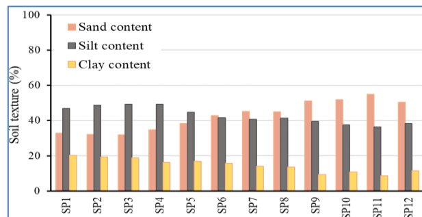
Fig. 2. Distribution of soil texture at all sampling positions across the study area.
