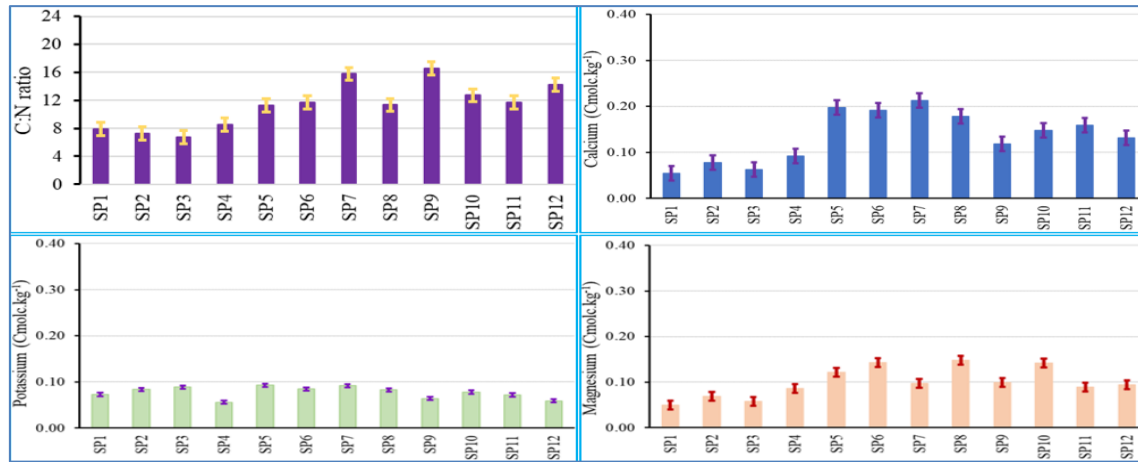
Fig. 4. Distribution of the C: N ratio and exchange ions at the investigated sampling positions in Lam River Basin.
