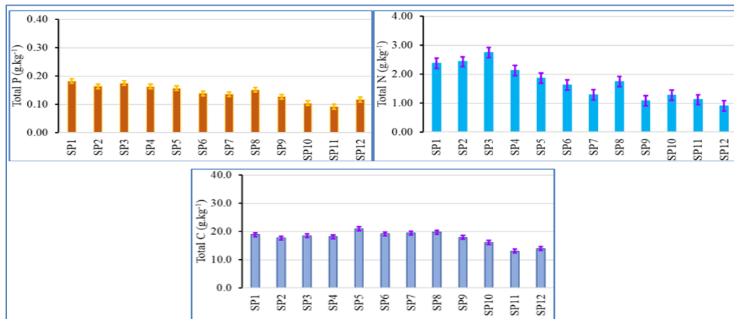
Fig. 5. Distribution of the soil organic contents at the investigated sampling positions in Lam River Basin.
