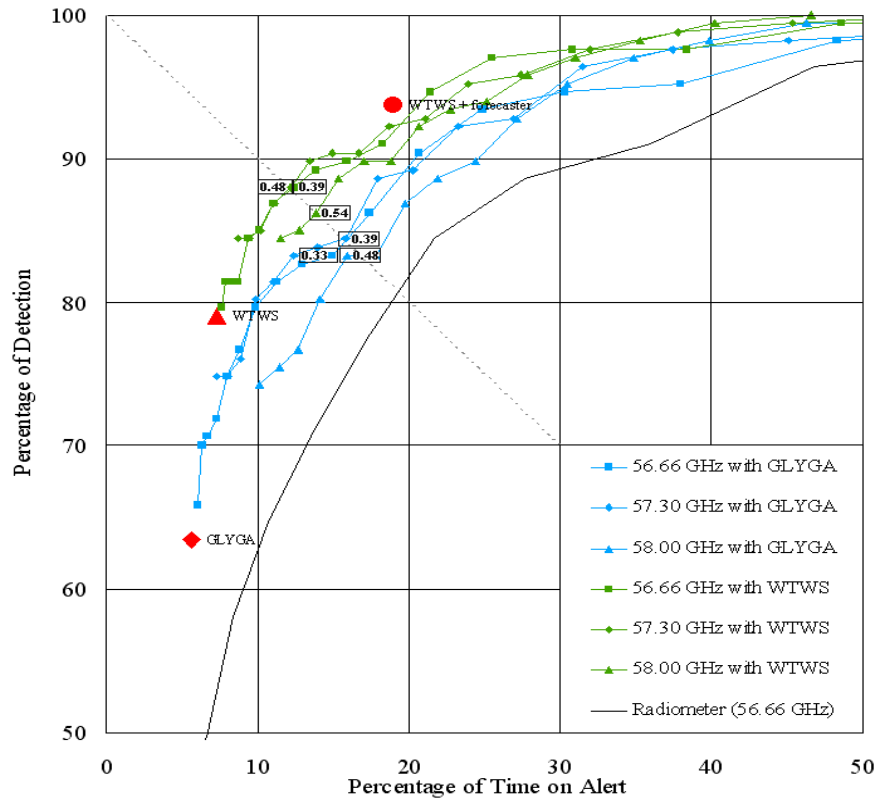
Fig. 6. Same as Fig. 4 but considering the windshear alerts based on the auto-correlation of three oxygen channels of the radiometer. The auto-correlation of two successive data points in each curve differs by 0.03. It ranges from 0.15 to 0.6 from right to left
