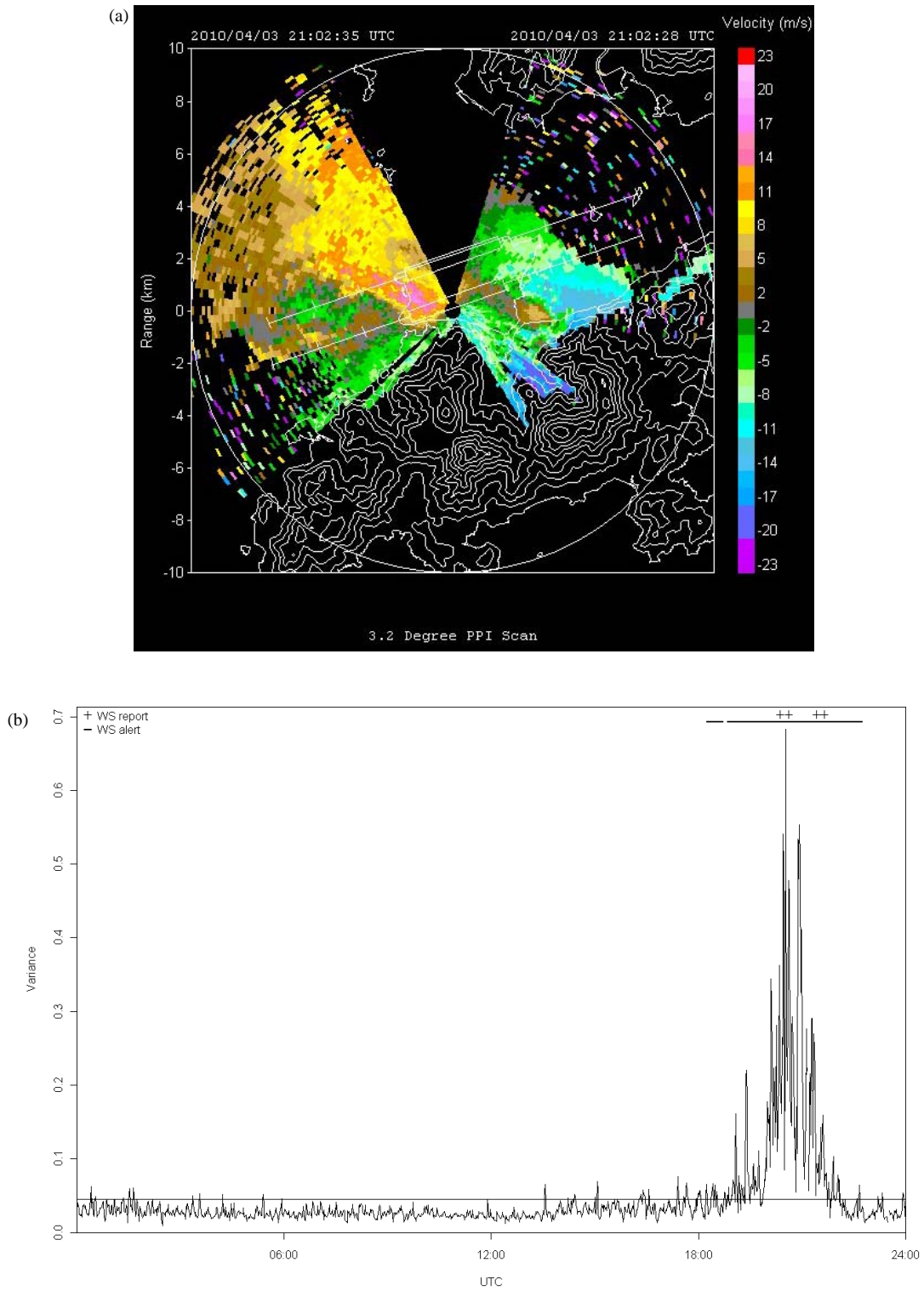
Figs. 2(a&b). (a) The radial velocity imagery of the south runway LIDAR for the case of terrain-induced windshear on 3 April 2010. (b) Time series of the variance of the brightness temperature at 57.3 GHz with the times of the pilot windshear reports shown in crosses. The effective height of 57.3 GHz is about several hundred metres (in the order of 400 m) above ground, which closely corresponds to the height of reporting of low-level windshear by the pilots
