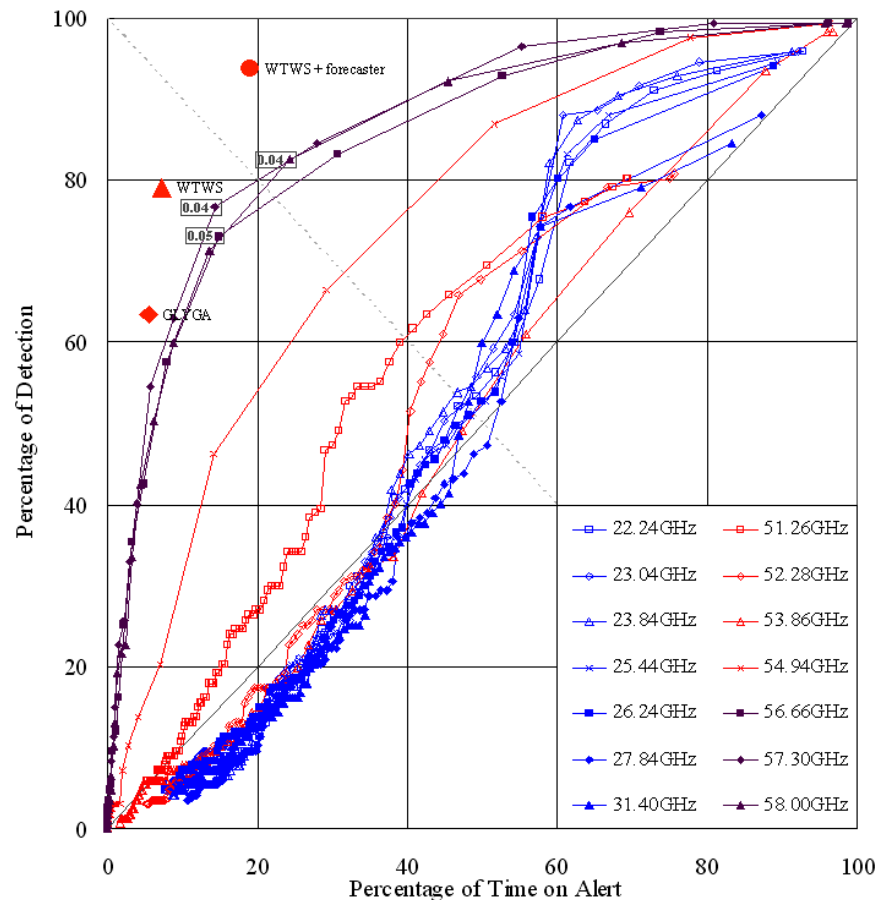
Fig. 3. The ROC curves of all the frequency channels of the microwave radiometer at HKIA. The variance of two successive data points in each curve differs by 0.005. It ranges from 0.005 to 0.5 from right to left with 100 data points. The performances of GLYGA, WTWS and overall windshear alerting service (WTWS + forecaster) are also shown
