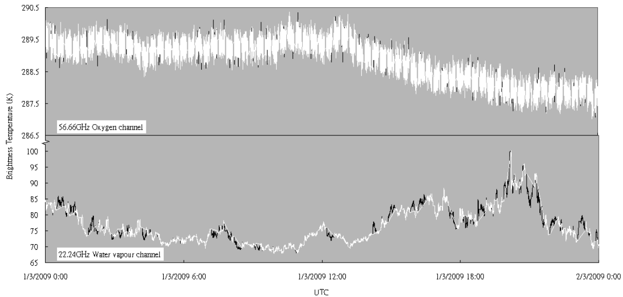
Fig. 1. Sample time series of the brightness temperature from an oxygen channel (upper) and a water vapour channel (lower). The raw brightness temperatures are shown in black, and the quality-controlled values are shown in white. The effective height of the oxygen channel considered here is several hundred metres (in the order of 400 m) above ground
