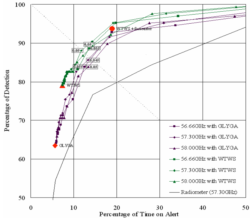
Fig. 4. The ROC curves by combining variance-based alerts of three oxygen channels (56.66 GHz, 57.3 GHz and 58.0 GHz) with GLYGA alerts, and by combining them with WTWS alerts. The variance of two successive data points in each curve differs by 0.005. It ranges from 0.035 to 0.1 from right to left in 20 data points
